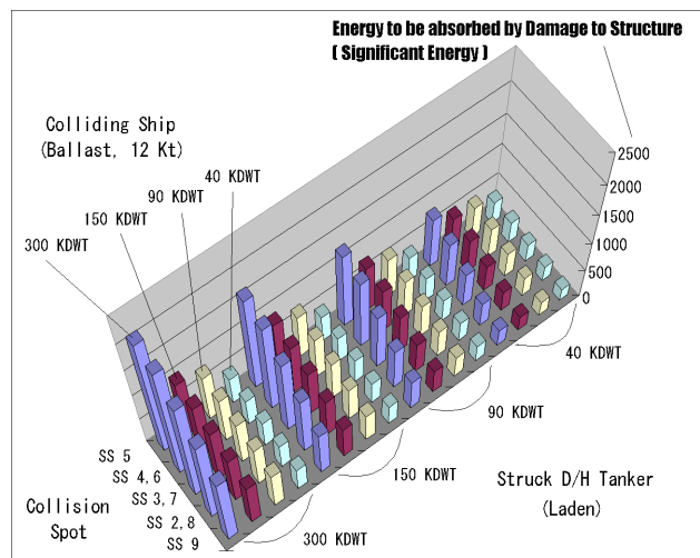
Fig-4-3 Energy to be absorbed by structural damage
