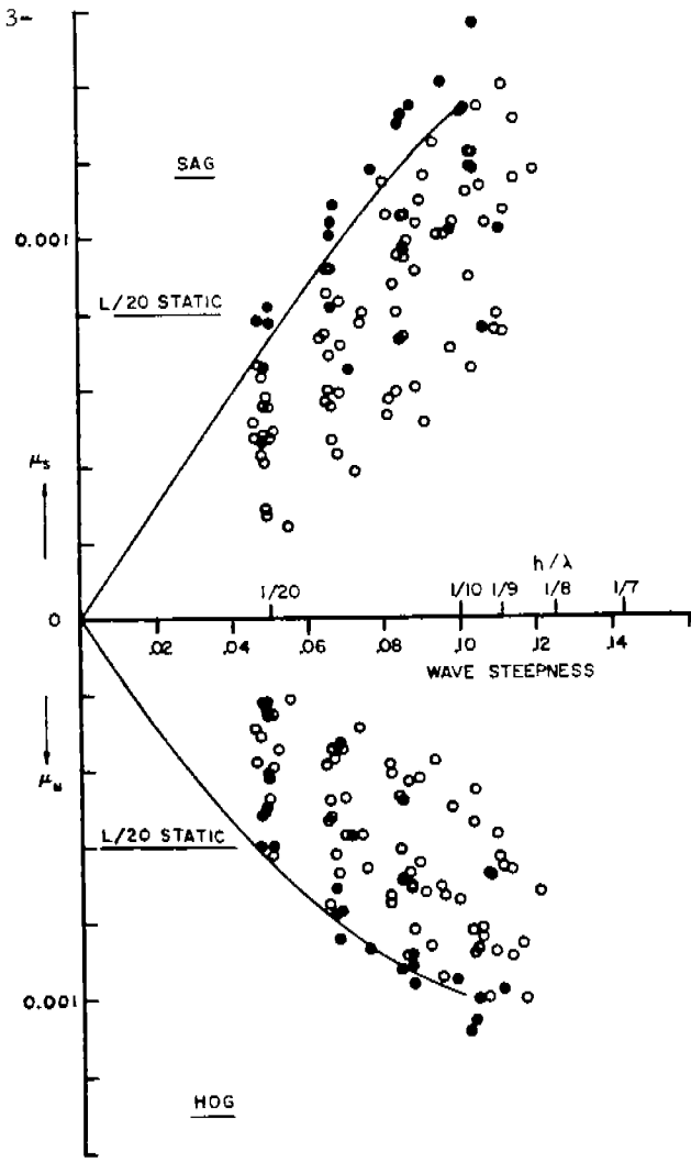
FIG. 15. MEASURED BENDING MOMENT DATA ---- ALL WAVE LENGTHS AND SPEEDS MODEL 2251A-V2; MARINER, CARGO AMIDSHIP.
