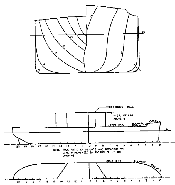
FIG. 5. MODEL DRAWING, MODEL 2251D - GIANT TANKER.
