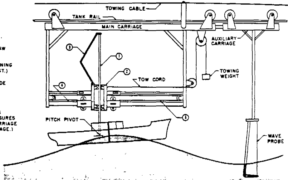
FIG. 2. SCHEMATIC OF TOWING APPARATUS.
