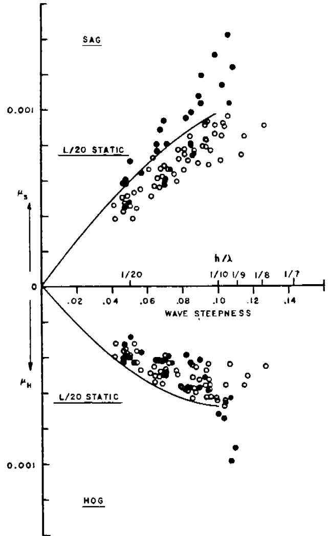
FIG. 19. MEASURED BENDING MOMENT DATA ---- ALL WAVE LENGTHS AND SPEEDS MODEL 2130; DESTROYER.
