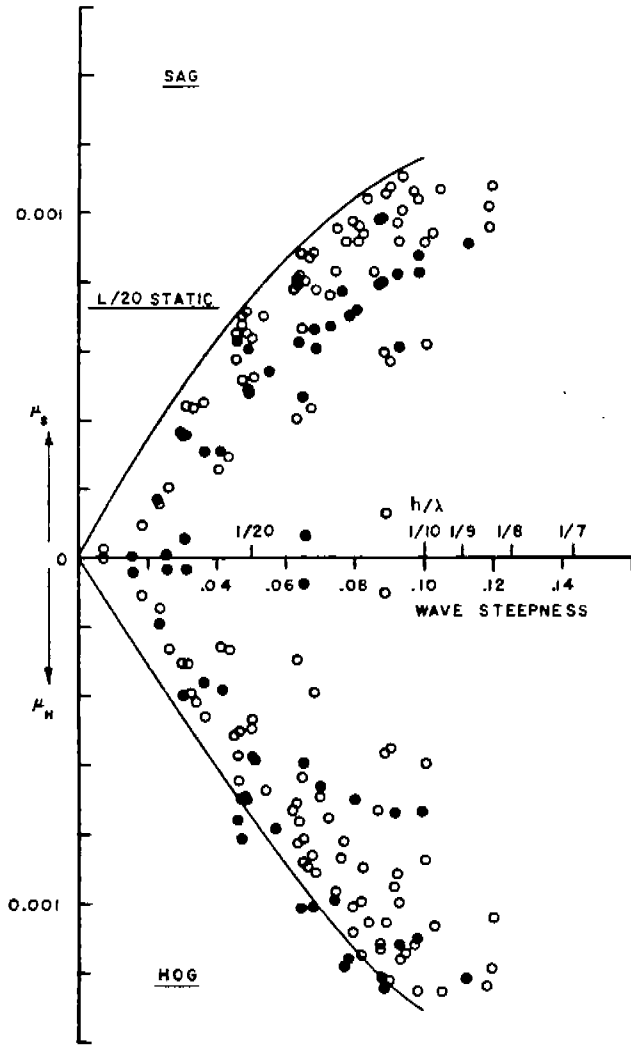
FIG. 18. MEASURED BENDING MOMENT DATA ---- ALL WAVE LENGTHS AND SPEEDS MODEL 2251D; GIANT TANKER.
