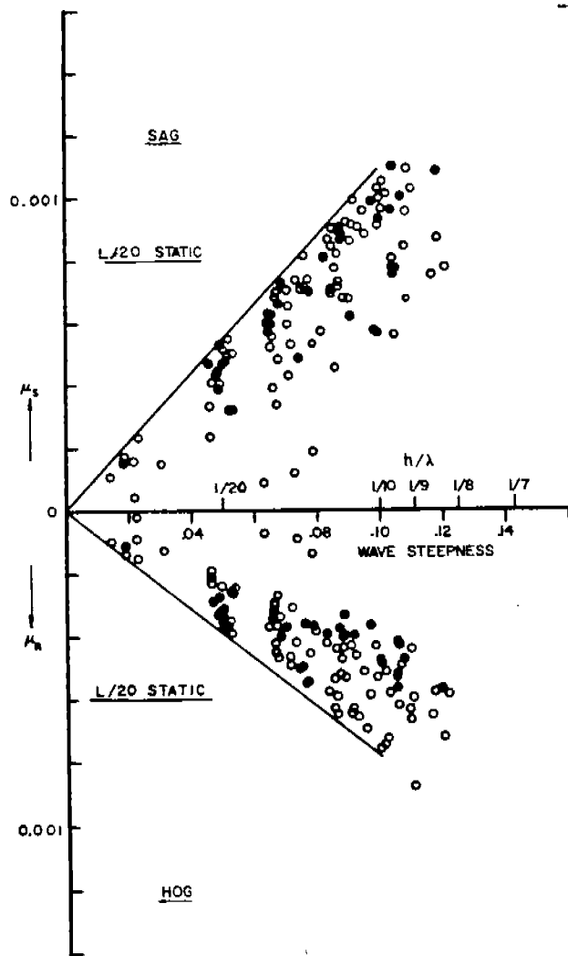
FIG. 14. MEASURED BENDING MOMENT DATA ---- ALL WAVE LENGTHS AND SPEEDS. MODEL 2251A-VI; PARENT MARINER.
