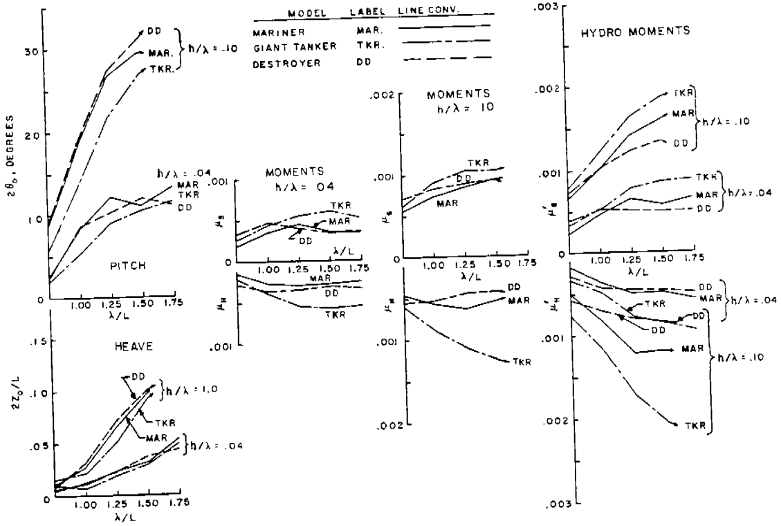
FIG. 12. CROSS PLOT OF FAIRED MOMENTS AND MOTIONS HEAD SEAS FROUDE NO. 0.0.
