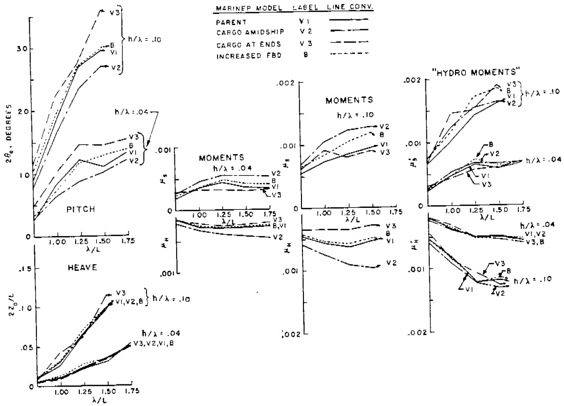
FIG. 11. CROSS PLOT OF FAIRED MOMENTS AND MOTIONS HEAD SEAS FROUDE NO. 0.0.
