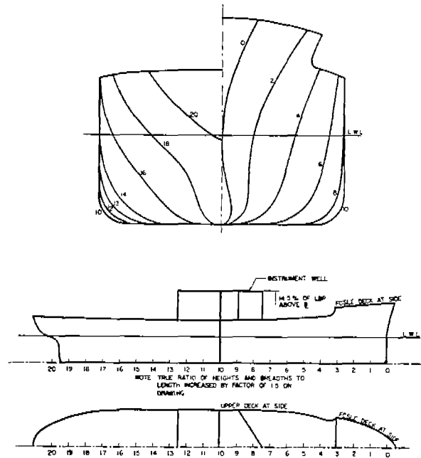
FIG. 4. MODEL DRAWING, BASIC MARINER HULL - MODELS 2251A-VI, 2251A-V2, 2251A-V3.
