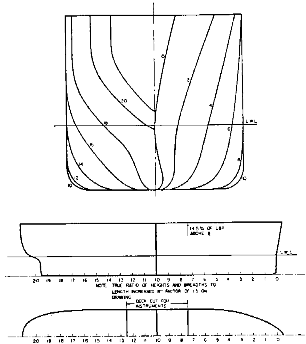
FIG. 7. MODEL DRAWING, MODEL 2251B - MARINER WITH INCREASED FREEBOARD.
