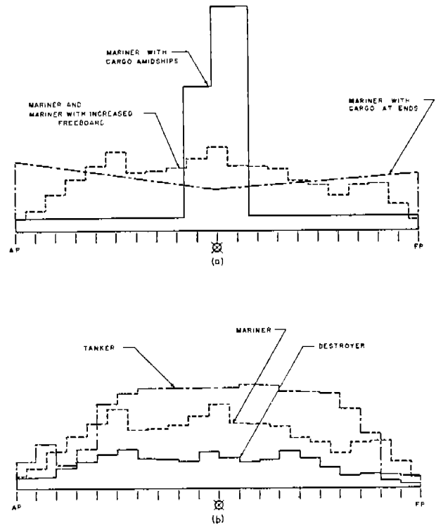
FIG. 8a and b. WEIGHT DISTRIBUTIONS.
